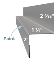
RPDA RP Double Angle
