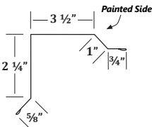
RR Residential Rake
