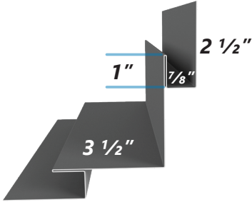
MBIC MB Inside Corner
