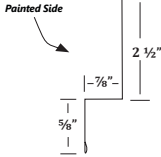
DA5 5/8" Double Angle
