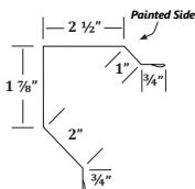
YL54 #54 Corner with 1-1/2" offset
