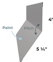
RPHSP RP High Side Parapet
