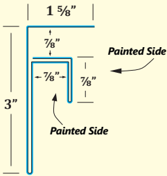
FJ7PI 7/8" F&J Painted Inside
