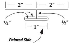
SD 3 Piece Soffit Divider
