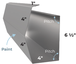
RPSCE RP Sculptured Eave
