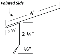
RDE Residential Drip Edge
