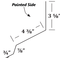
EWO Endwall with Offset
