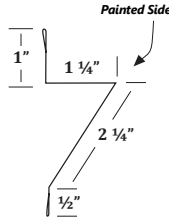
SG Snow Guard
