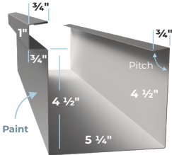
RPBE RP Box Eave
