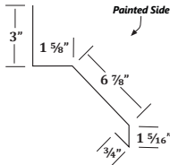
TC Track Cover Round FM
