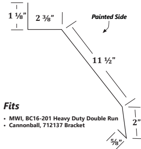
TCDH Track Cover Double Heavy Duty Round FM
