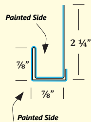
JPI J-Channel Painted Inside
