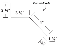
TCTM Track Cover Round TM
