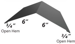
SL6RC SL 12" Ridge Cap
