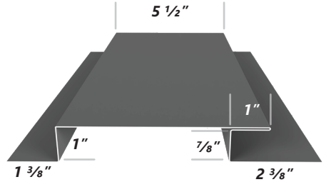
MBBB512 MB 5 1/2" Band Board
