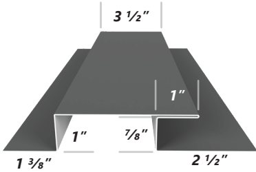
MBBB312 MB 3 1/2" Band Board
