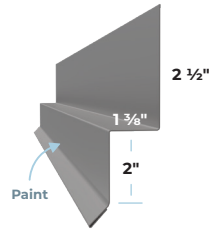
RPWT RP Wainscot Trim
