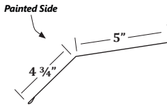
UG Upper Gambrel
