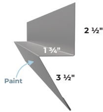
RPBA RP Base Angle
