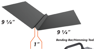
SL6VA SL 20" Valley
