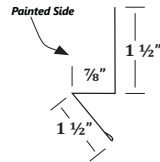
RG Rat Guard
