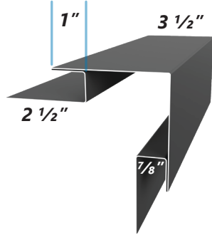
MBBB512 MB 5 1/2" Band Board
