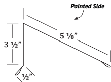
HS High Side Trim
