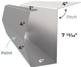
RPBHO RP Box Hang-On
