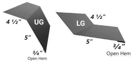
SL6LG SL Lower Gambrel
