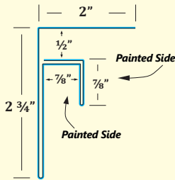
FJPI 1/2" F&J Painted Inside
