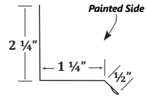
WD Window Drip Cap
