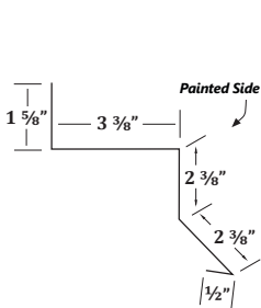
TCSTM Track Cover Square TM
