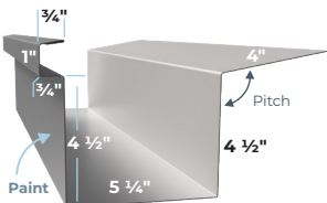
RPBE RP Box Eave
