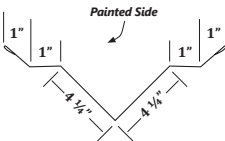
IC 6" INSIDE Corner
