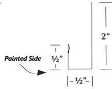
SJ Soffit J-Channel
